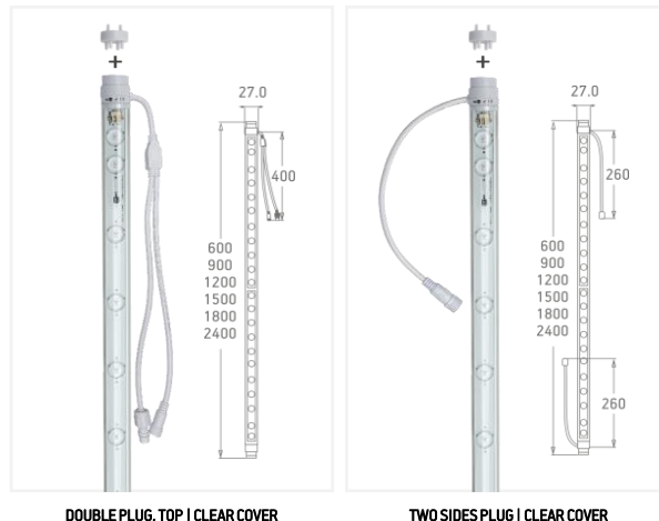
DOUBLE PLUG, TOP | CLEAR COVER
