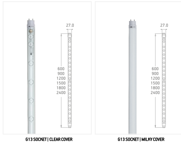
G13 SOCKET | CLEAR COVER
